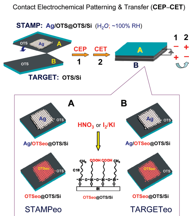
Figure 1. Schematic representation of the parallel CEP–CET process. (See the text.) The lower panel shows transferred and residual silver patterns on surface B (electrooxidized target—TARGETeo) and surface A (electrooxidized stamp—STAMPeo), respectively, and the corresponding monolayer prints (OTSeo@OTS/Si) revealed under the silver features upon removal of the metal from both surfaces with \text{HNO}_3 or \text{I}_2/\text{KI} .
