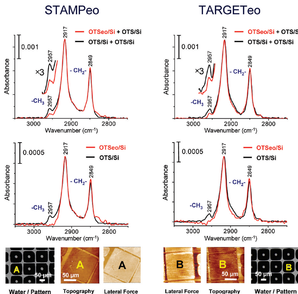
Figure 3. Quantitative micro-FTIR spectra (C–H stretching spectral region) acquired (with a 75 μm × 75 μm microscope aperture) from OTSeo/Si monolayer prints within square A of STAMPeo (left column) and square B of TARGETeo (right column) in the monolayer patterns displayed in Figure 2 (bottom) and from unaffected OTS/Si regions of the respective monolayer/silicon specimens. All displayed curves represent net spectral contributions of the respective organic monolayers, after mathematical subtraction of the spectral contributions of the corresponding bare silicon substrates. The notation OTSeo/Si + OTS/Si and OTS/Si + OTS/Si (in the top row curves) indicates the fact that, being recorded in transmission through double-side-polished silicon wafer substrates coated with an OTS monolayer also on their unmodified back sides, each of these spectral curves also contains the contribution of the respective back-side OTS/Si monolayer. The bottom-row curves show the corresponding net spectral contributions of each patterned front-side monolayer obtained by mathematical subtraction of the spectral contributions of the respective unmodified back-side monolayer (based on the fact that monolayer films assembled on each side of a double-side-polished wafer are identical). Spectra collected with an elongated rectangular aperture from hydrophobic bar regions separating the hydrophilic squares of the pattern (not shown) confirm that these consist of the unmodified OTS monolayer. Optical micrographs of water condensation patterns employed in the visualization of the monolayer patterns and the focusing of the FTIR microscope aperture on the desired surface sites 14 are shown below the respective spectral curves along with complete SFM images of squares A and B.
