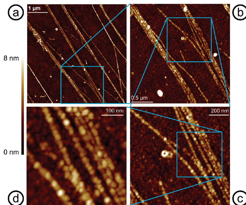
Figure 3. Noncontact mode AFM topography images showing a sample that was prepared by spin-coating a 1:10 silk solution. The images show self-assembly of silk protein into linear, thread-like structures.
