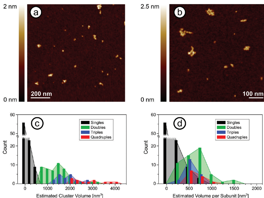
Figure 1. (a, b) Noncontact AFM topography images from native silk molecules (SF) deposited on a cleaved mica surface from a 1:1000 diluted solution without shear. The smaller features are round, have a diameter of 20–25 nm, a height of about 1.2 nm, and are most likely individual silk proteins. The larger objects are clusters of several proteins. (c) Histograms showing the volumes of proteins and protein clusters determined from AFM topography data. (d) Same as (c), except that volumes were divided by the number of apparent subunit within each cluster.
