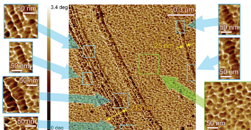
Figure 4. Noncontact AFM phase image of the same sample shown in Figure 3. Areas in colored boxes are featured with higher magnification on the left and right sides of the main image. The majority of the sample looks like the area highlighted in the green box: unorganized, round protein molecules. The blue boxes highlight areas in the nanofibrils featuring anisotropic conformation of the proteins. Sections across a single nanofibril and a bundle of nine nanofibrils are indicated in yellow.
