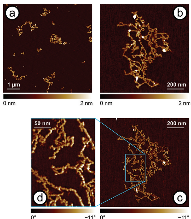
Figure 5. Noncontact AFM images of silk deposited from an aqueous 1:1000 solution by spin-coating, which induced shear in the solution: (a, b) topography image; (c, d) phase images. The proteins self-assemble into nanofibrils. The diameter is less than one of the globular single proteins shown in Figure 1, which were deposited from the same solution. This indicates that the protein undergoes conformational changes during the spin-coating process.
