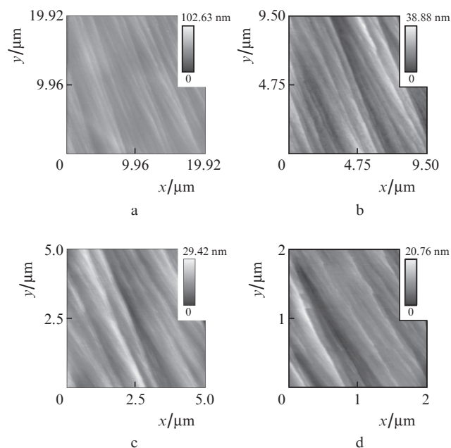
Figure 3. AFM images of a fracture surface of the Tm:CaF 2 ceramic at different magnifications.
