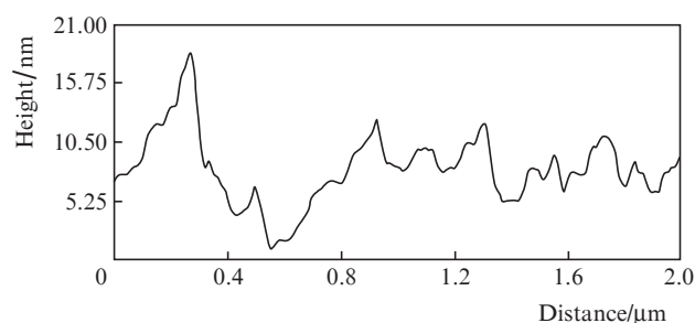
Figure 4. Surface profile in a section normal to the layer direction in a Tm:CaF 2 ceramic sample.
