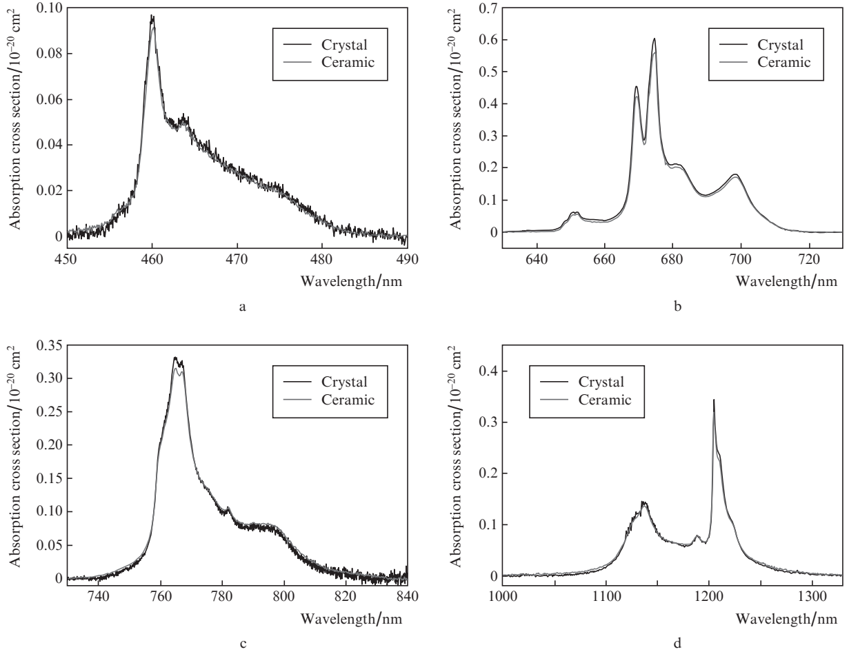
Figure 5. 300-K absorption spectra of the Tm:CaF 2 crystals and ceramic: (a) ^3\text{H}_6 \rightarrow ^1\text{G}_4 , (b) ^3\text{H}_6 \rightarrow ^3\text{F}_2 + ^3\text{F}_3 , (c) ^3\text{H}_6 \rightarrow ^3\text{H}_4 and (d) ^3\text{H}_6 \rightarrow ^3\text{H}_5 transitions.
